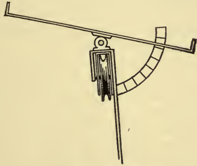
FIG. 138.—Gun-sight attachment to the perimeter to assist in bringing the center of the eye to the center of the arc.
